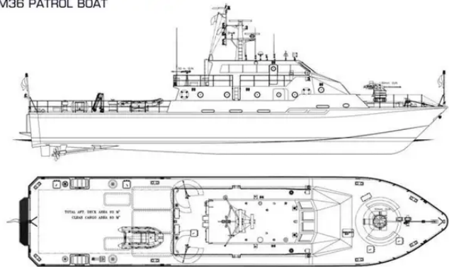
M36 PATROL BOAT
